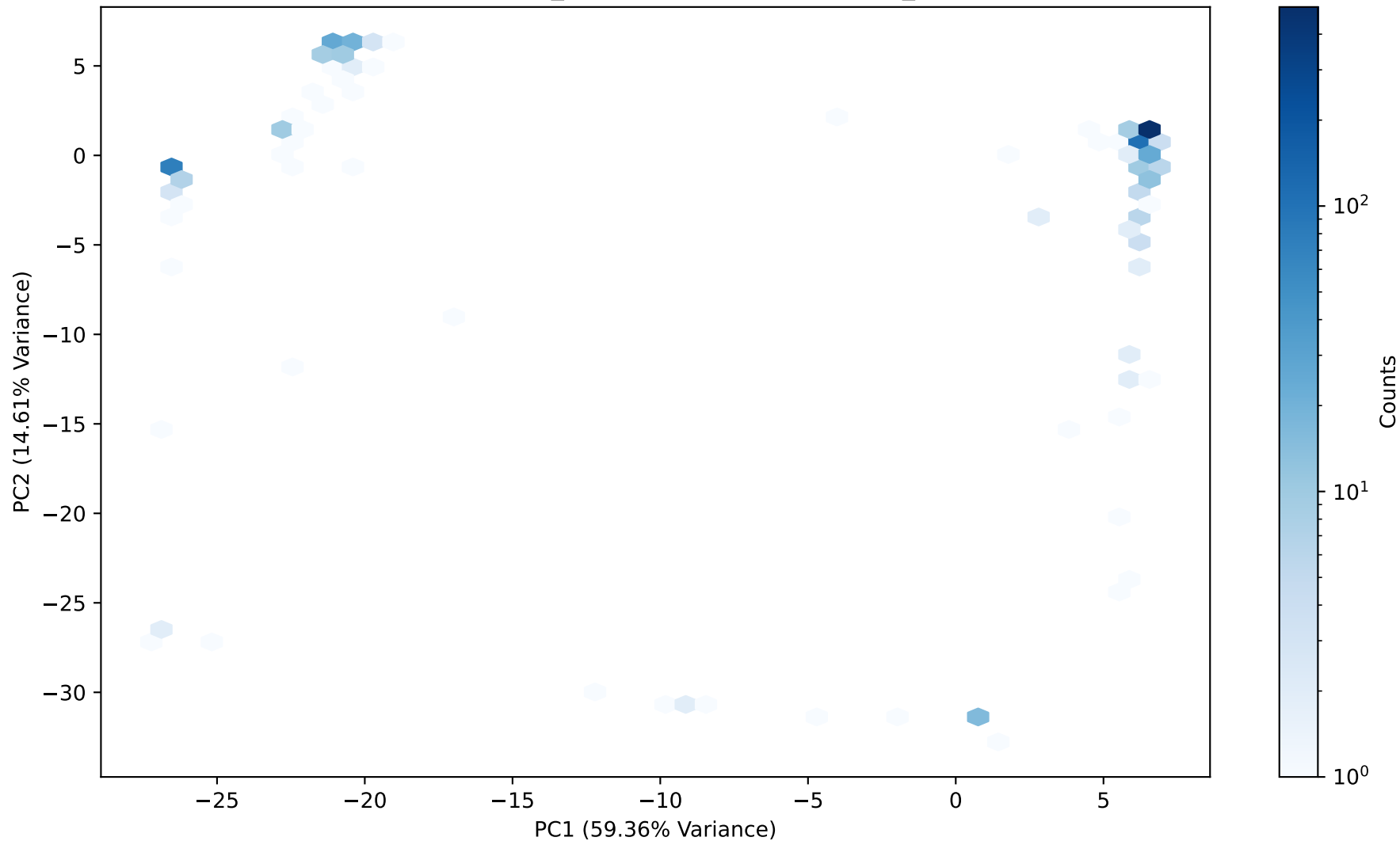
PCA of Alignment is_match Matrix - unassigned_circular
