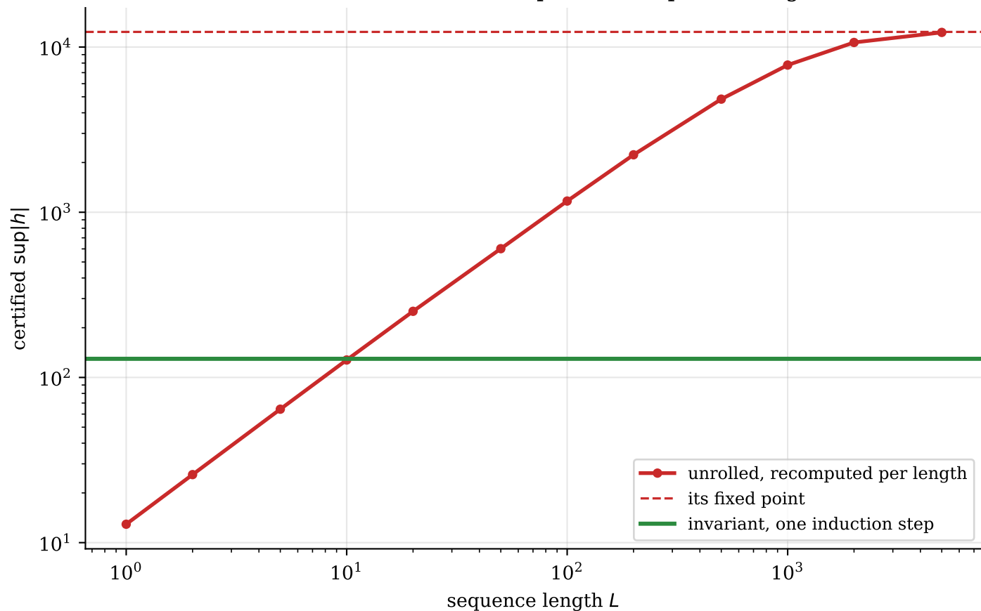
The invariant does not depend on sequence length
