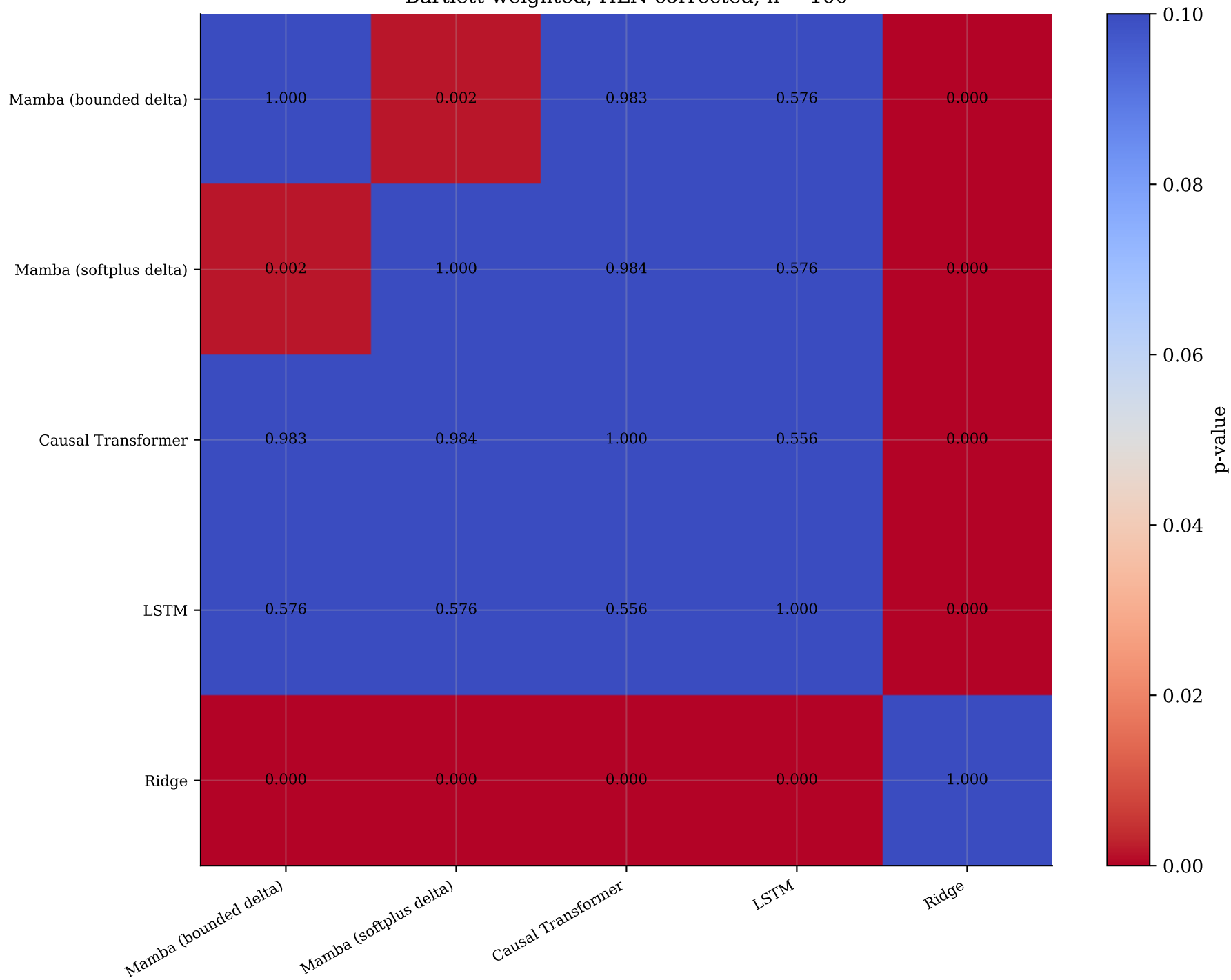
Diebold-Mariano p-values Bartlett-weighted, HLN-corrected, h = 100
