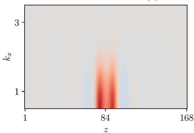
GENE reference \text{Re}[\tilde{g}]
