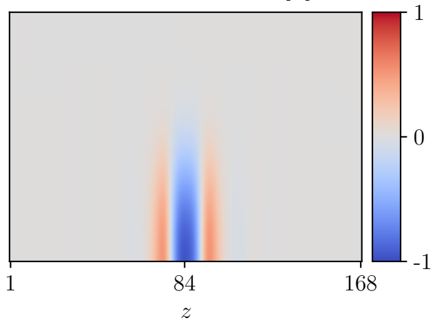
GENE reference \text{Im}[\tilde{g}]
