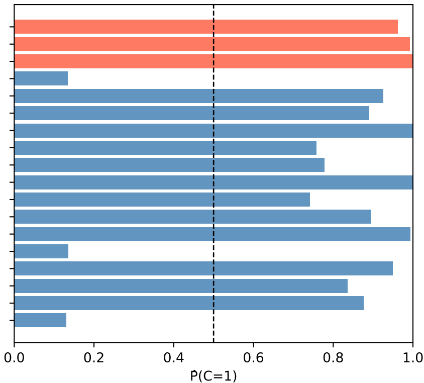
Old Gibbs (logistic C) acc = 0.333
