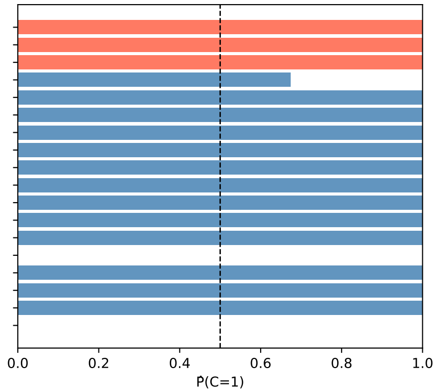
Collapsed Gibbs acc = 0.278
