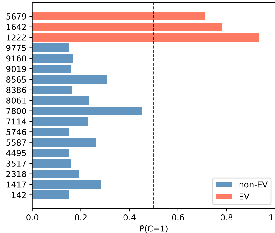
Heuristic acc = 1.000
