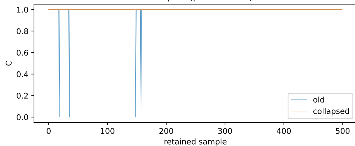
C samples (post burn-in)
