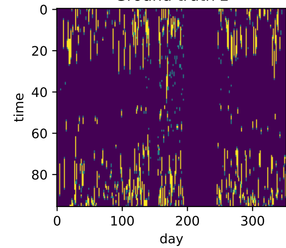
Ground truth z
