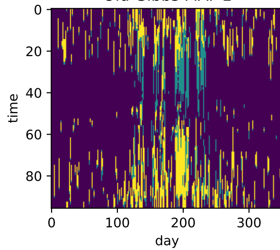
Old Gibbs MAP z
