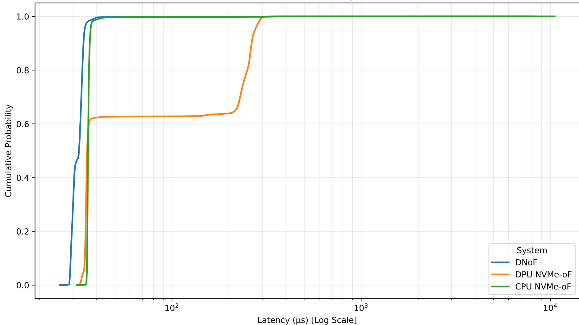
CDF of I/O Total Latency (Q→C)
