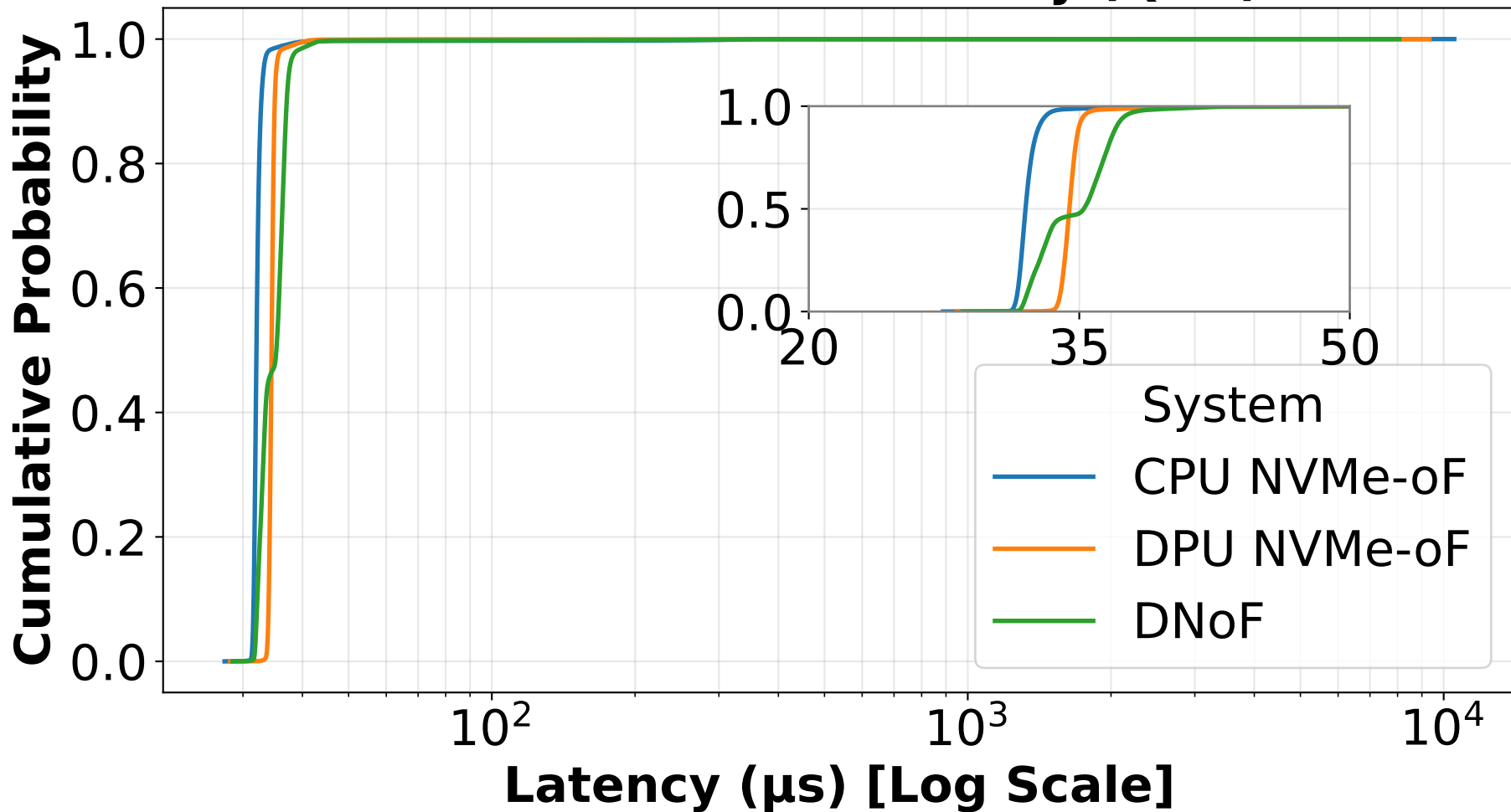
CDF of I/O Total Latency (Q→C)
