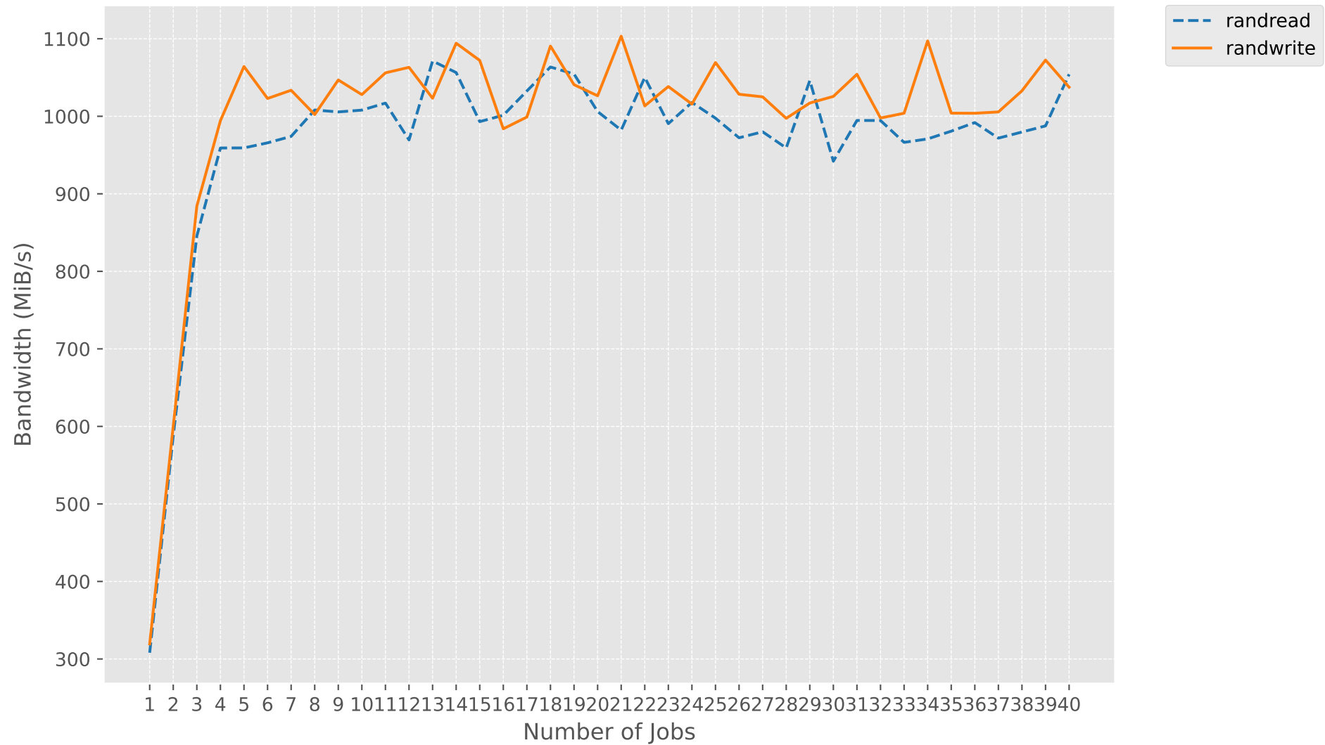
Bandwidth vs numjobs
