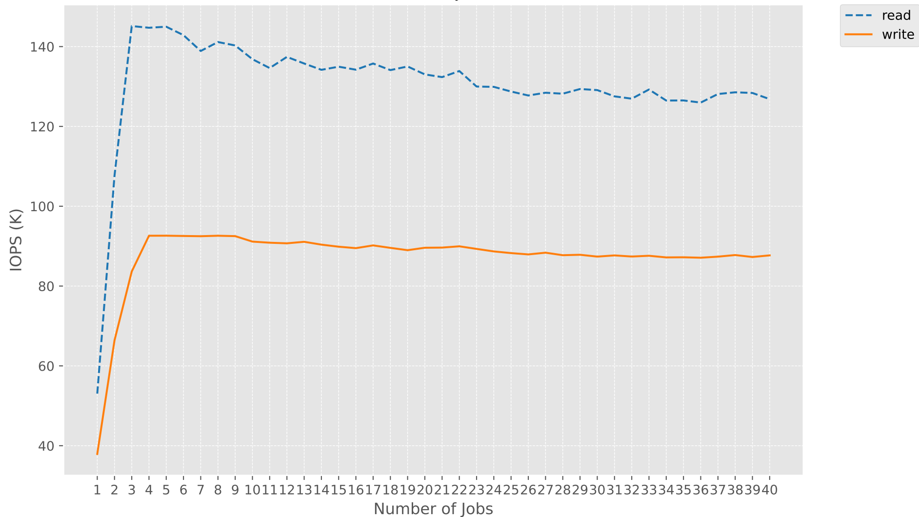
IOPS vs numjobs-bw
