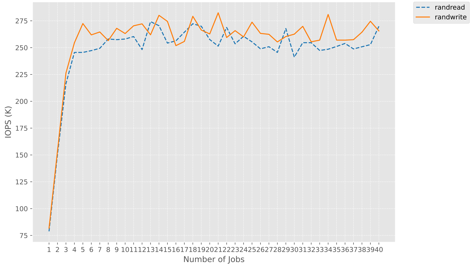
IOPS vs numjobs
