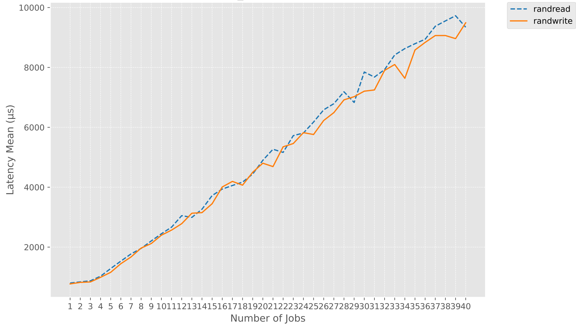
Latency_Mean vs numjobs
