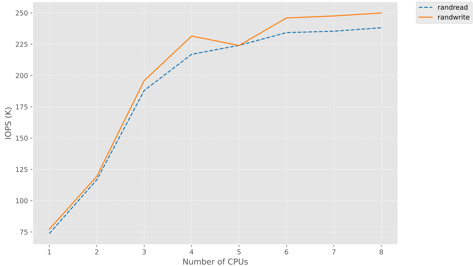
IOPS vs NBCPU
