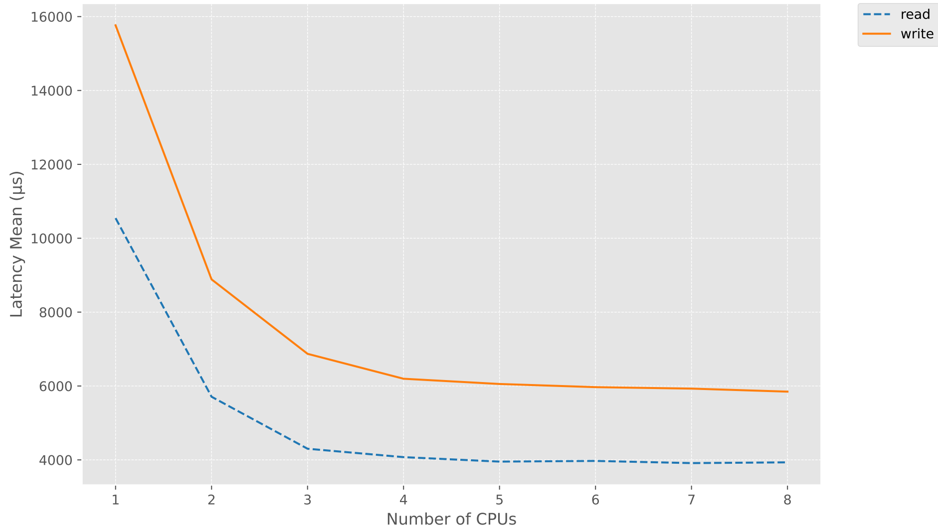
Latency_Mean vs NBCPU-BW
