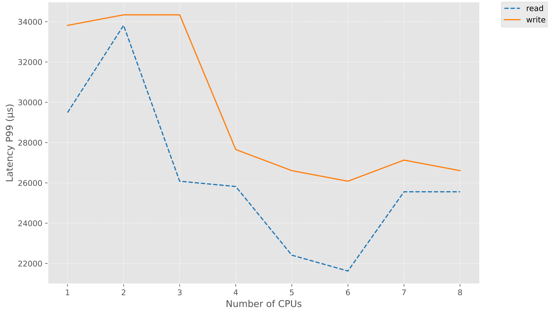
Latency_P99 vs NBCPU-BW
