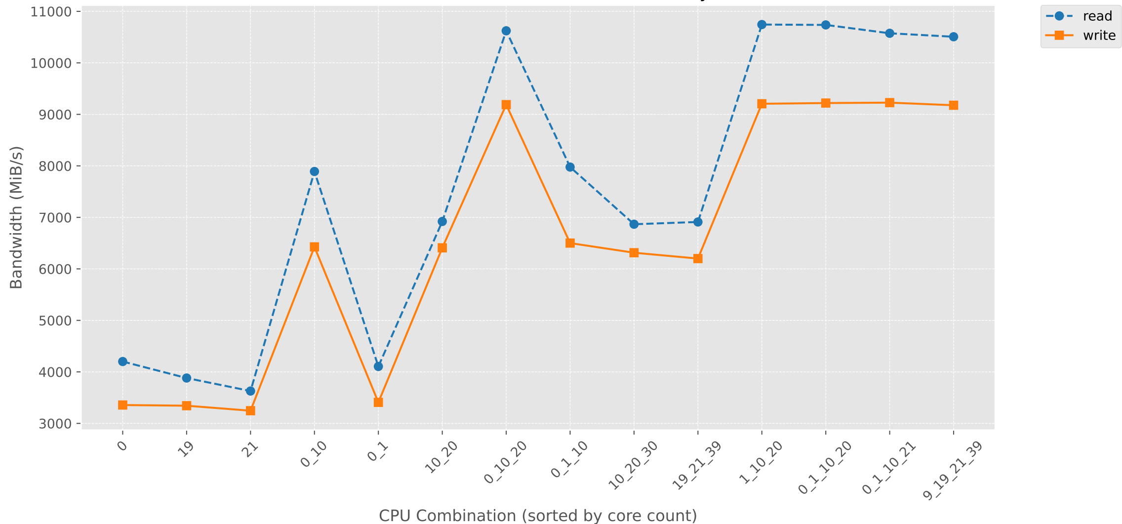
Bandwidth vs NBCPU-BW (CPU Affinity)
