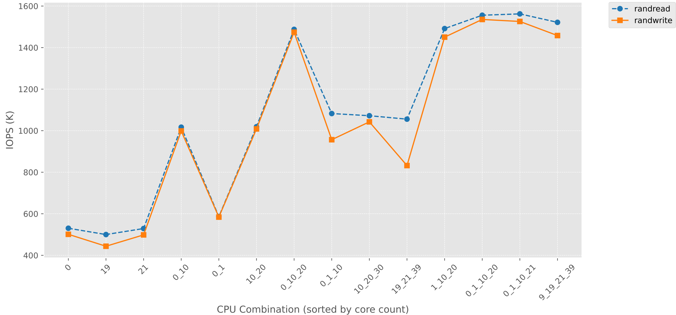
IOPS vs NBCPU-RAND (CPU Affinity)
