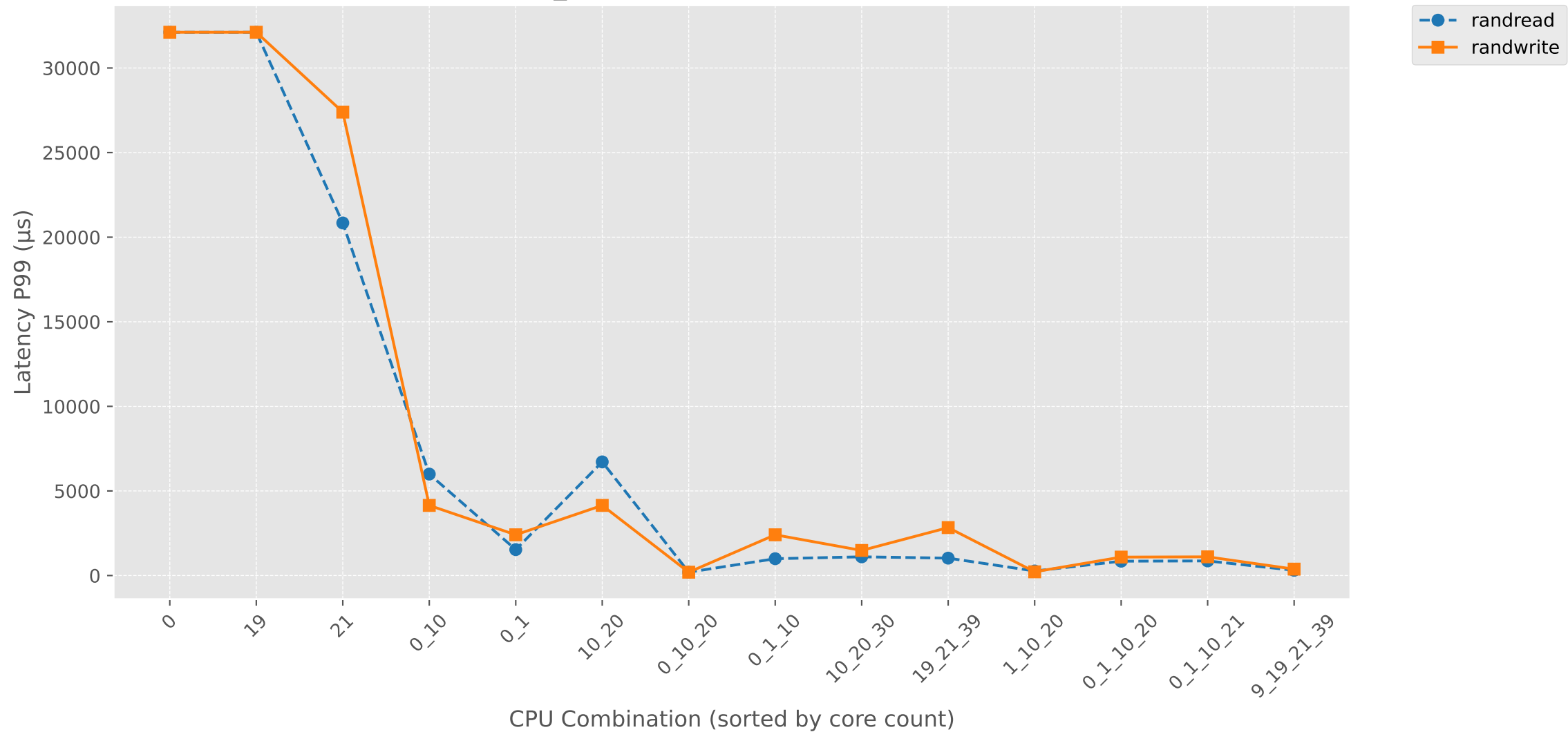
Latency_P99 vs NBCPU-RAND (CPU Affinity)
