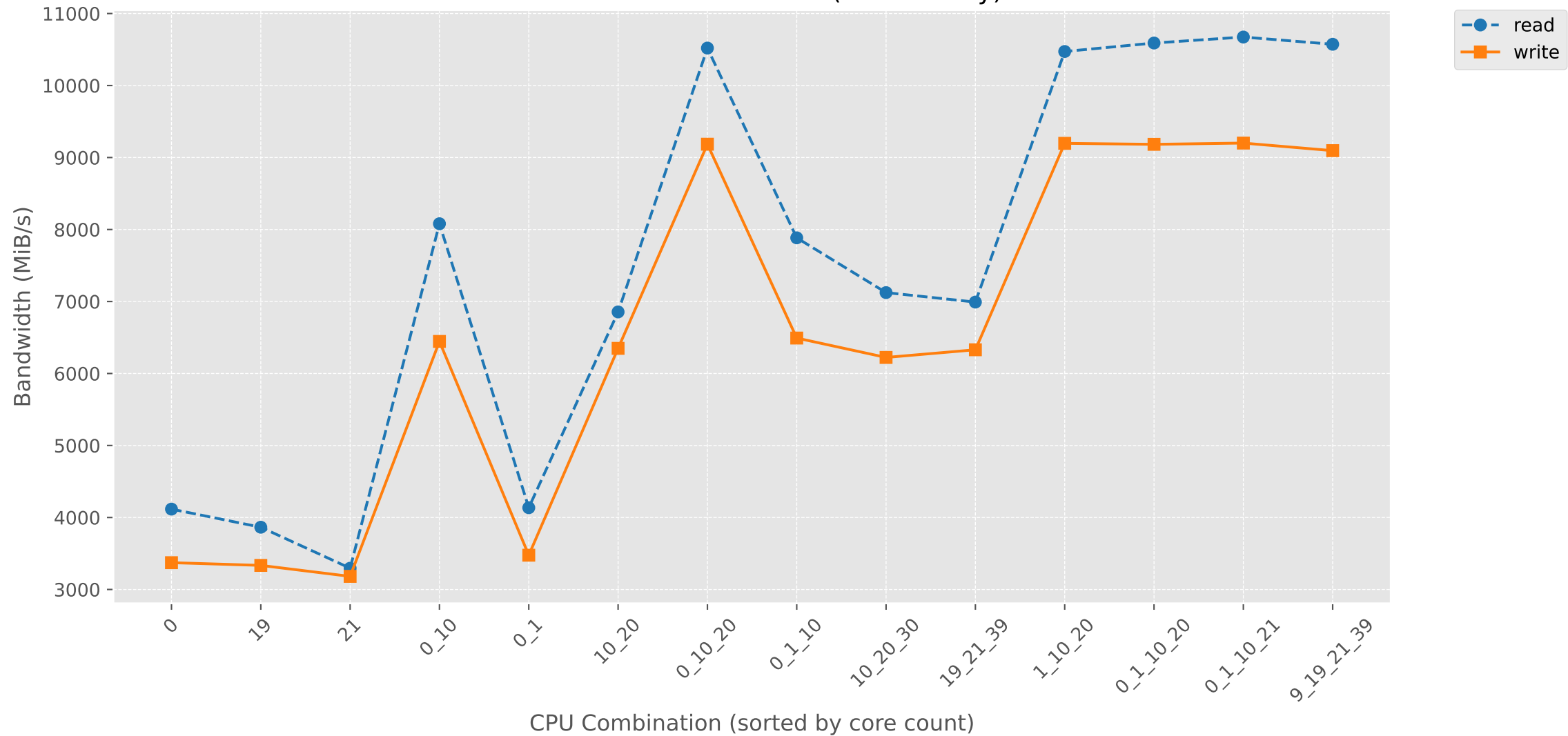
Bandwidth vs NBCEP-BW (CPU Affinity)
