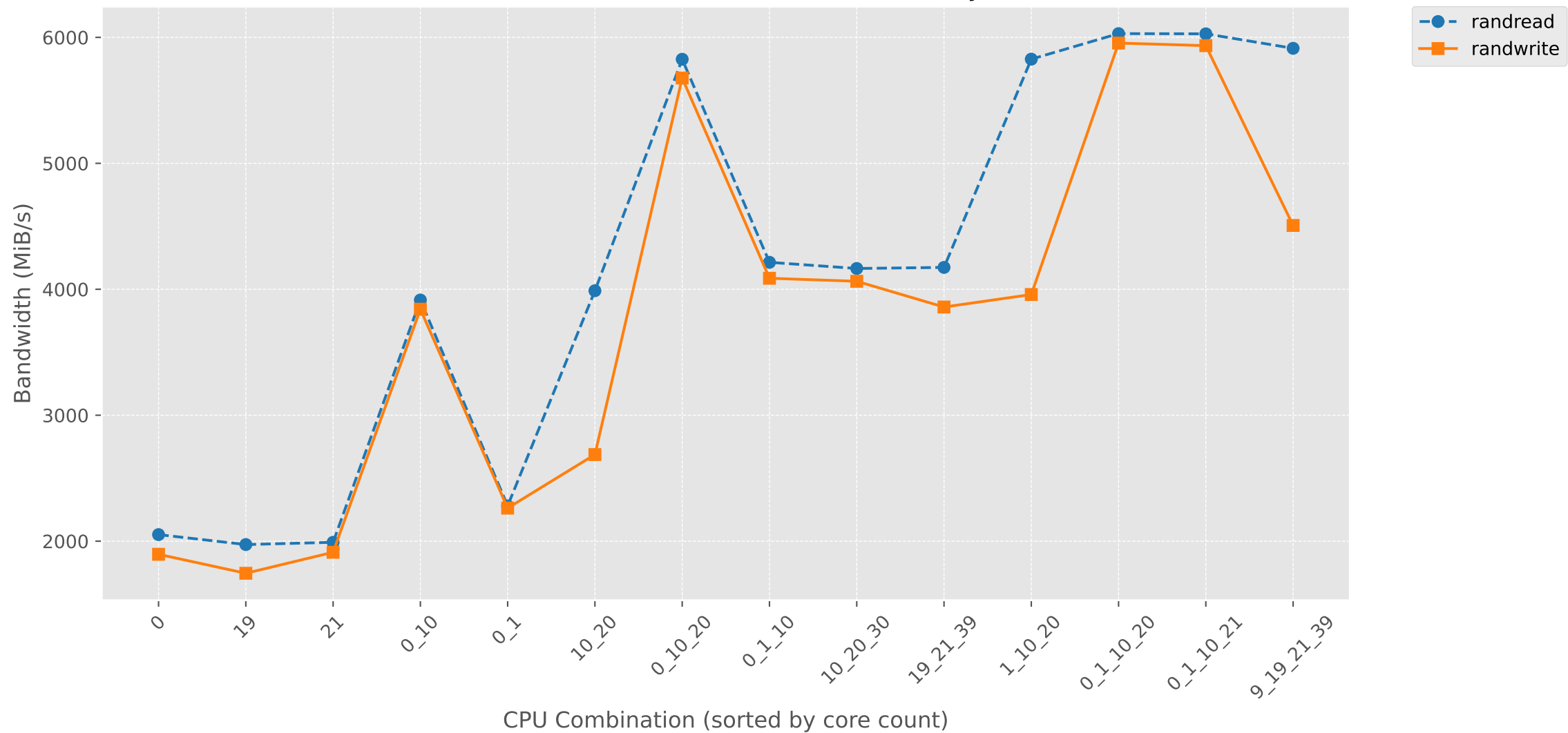
Bandwidth vs NBCCPU-RAND (CPU Affinity)
