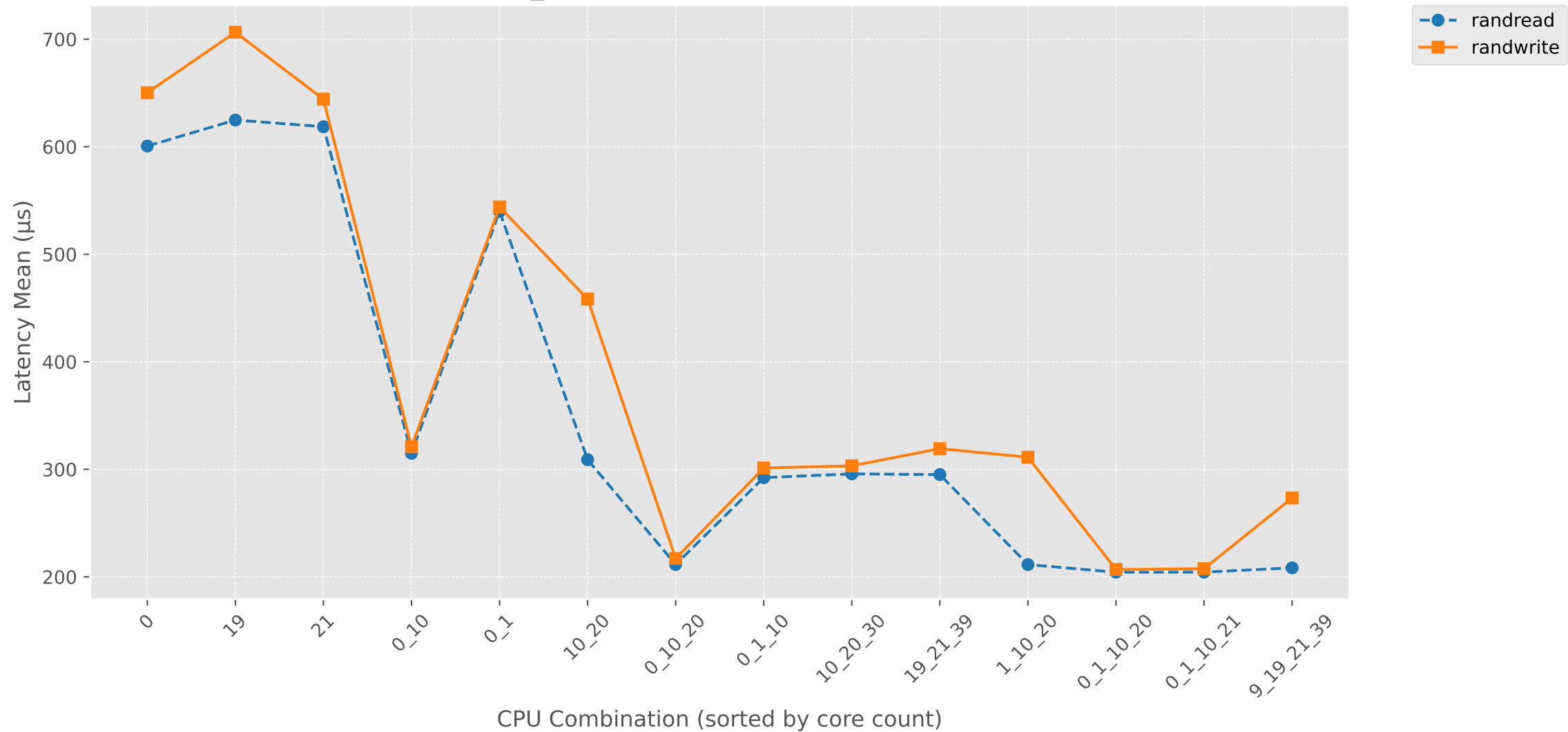
Latency_Mean vs NBCPU-RAND (CPU Affinity)
