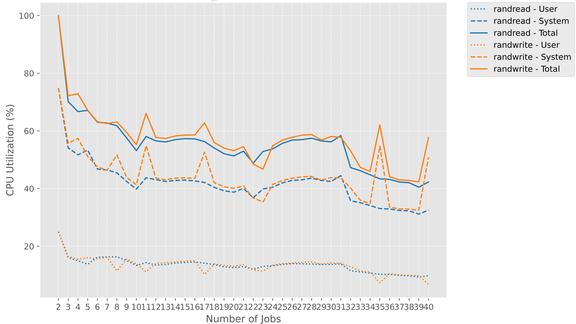
CPU_Total vs nbcpu
