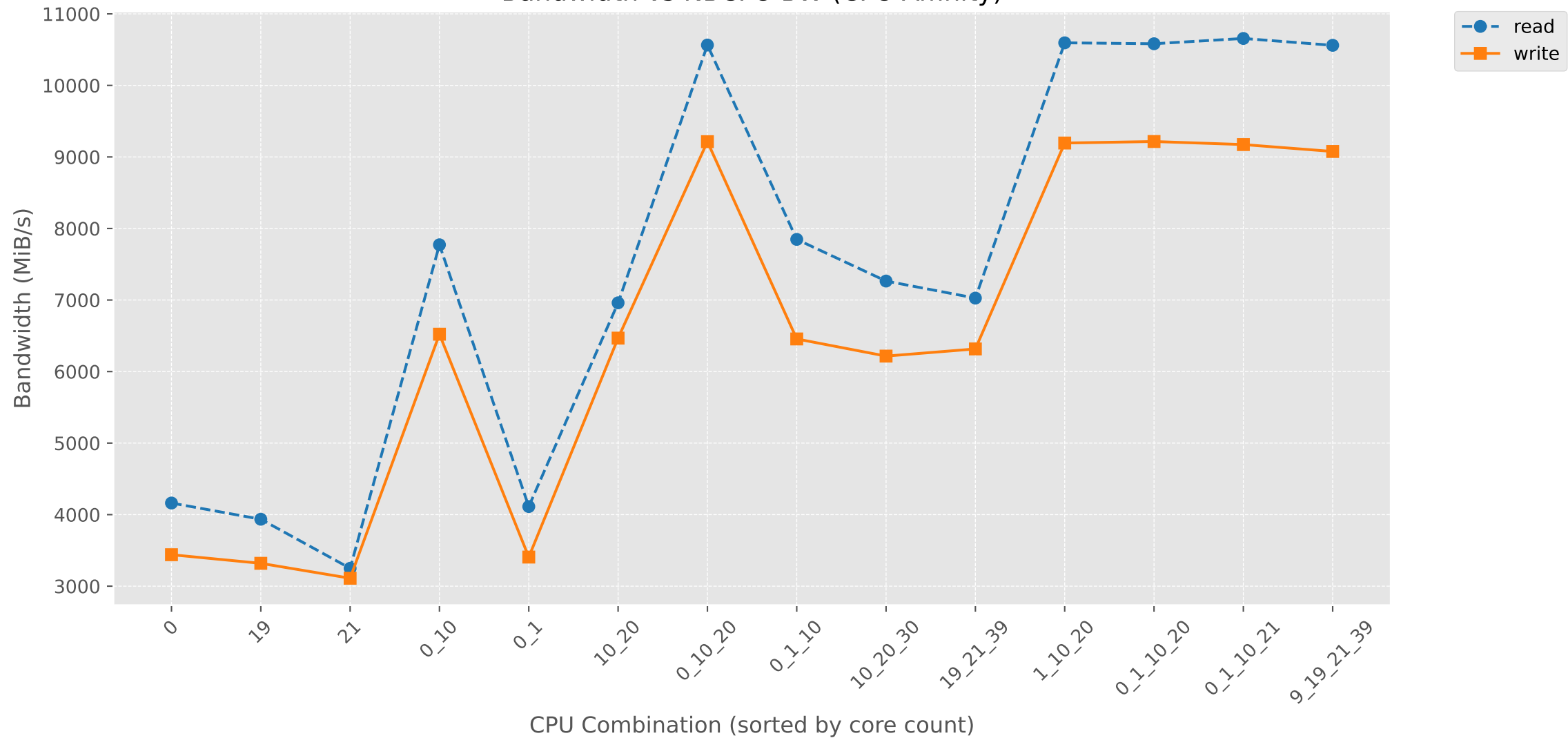
Bandwidth vs NBCCPU-BW (CPU Affinity)
