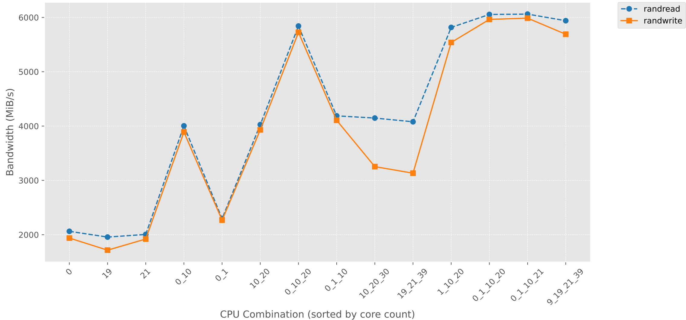
Bandwidth vs NBCPU-RAND (CPU Affinity)
