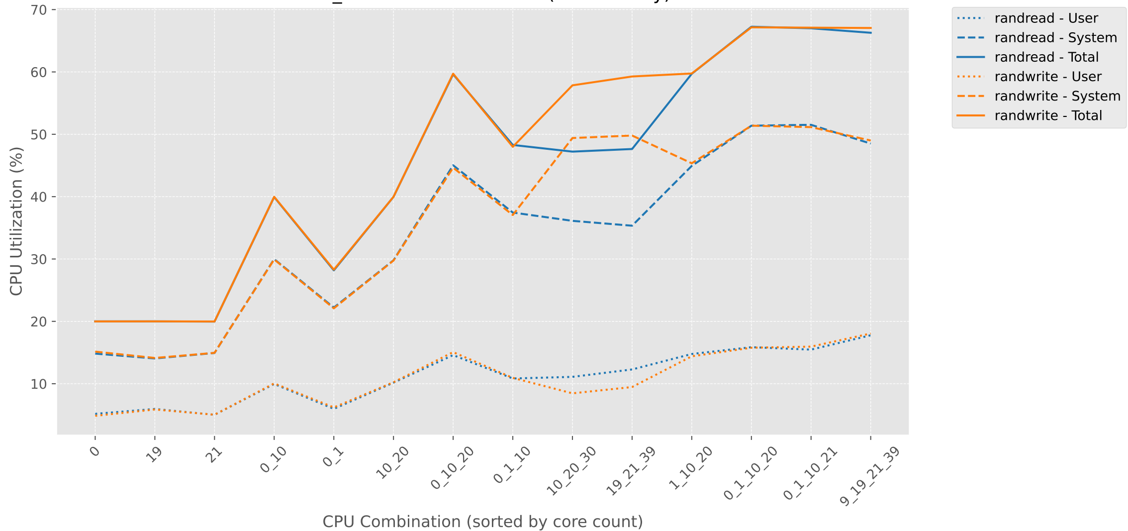
CPU_Total vs NBCPU-RAND (CPU Affinity)
