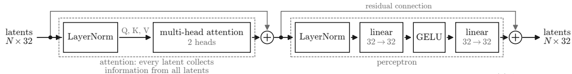
(b) self-attention layer, \times 3
