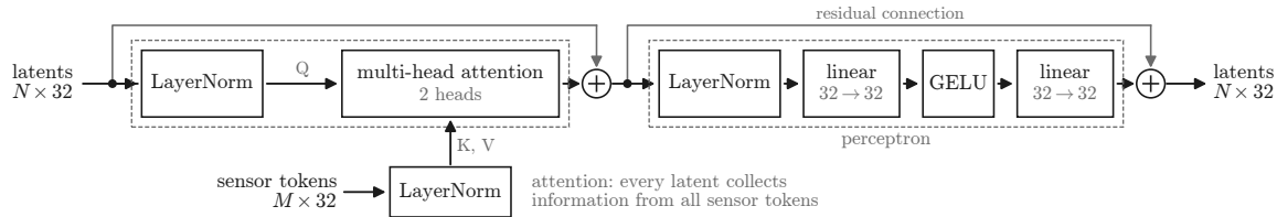
(a) cross-attention layer
