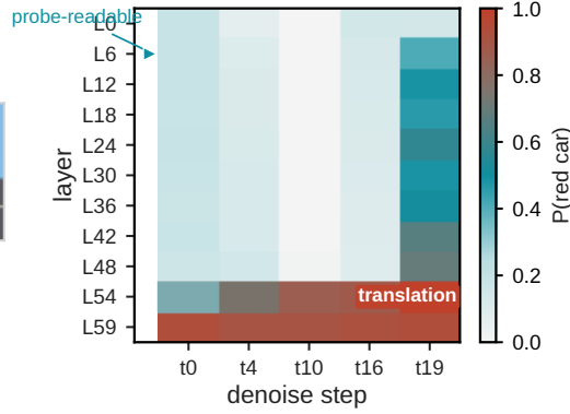
Figure 1: Predictable early, translated late. A: source and realized edit. B: frozen-head P(\text{red car}) across layer and step; the outcome is probe-readable at L6, but translation into the head-readable velocity convention occurs at L52–54. C: the five measured stages used throughout the paper.
