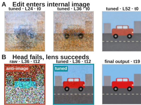
Figure 4: Internal image vs. frozen-head ghost. A: the tuned lens (fit on non-color edits, zero-shot on car_red ) shows the edit entering a coherent internal image at t=0 : L24 retains the source-blue car, L36 turns it orange-red, and L52 resolves the edited scene. Because the sampled pixels are pure noise at this step, the image comes from the decoded internal code. B: on the identical L36/ t=12 state, the frozen head produces a cyan-car anti-image while the tuned lens recovers the coherent red-car scene; the final output is shown for reference.
