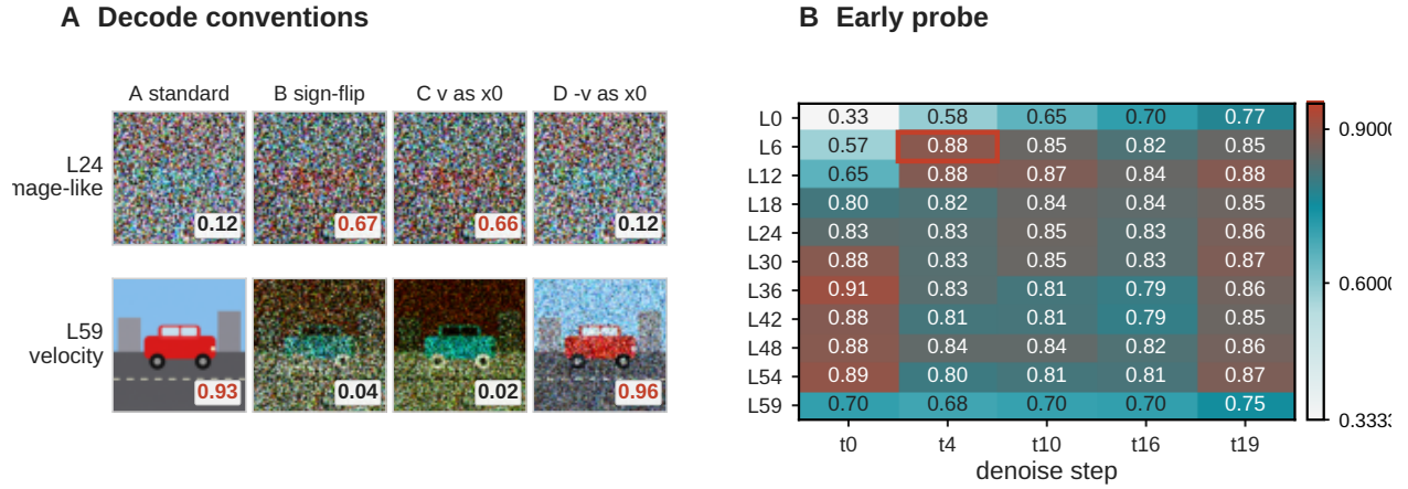
Figure 3: Decode convention flips; the probe reads early. A: four decodes of car_red at t=4 ; the image-like and standard conventions reverse between L24 and L59. B: 3-way probe accuracy (chance 0.33); the outlined L6/t4 cell reaches 0.883 while the frozen head at the same state still reads noise. Red score pills in A mark target probability above 0.5.
