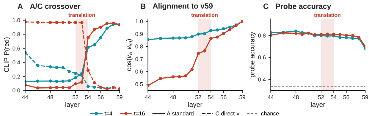
Figure 5: Translation band L52–54. Dense L44–L59 sweep on car_red . A: standard vs. direct- v CLIP scores cross in the same band at t=4 and t=16 (midpoints 52.7 and 53.6). B: \cos(v_t, v_{59}) rises sharply in that neighborhood. C: probe accuracy stays flat through L58 and drops at L59 only, separating translation from the terminal loss of linear readability.
