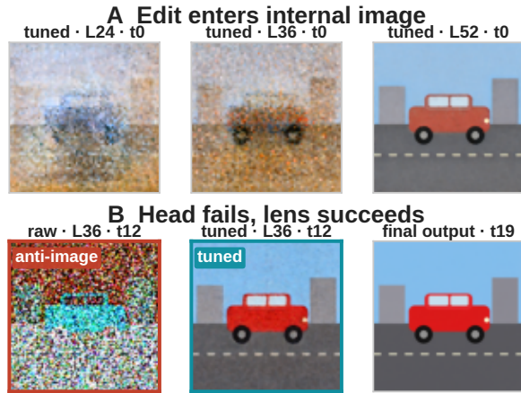
Figure 5: Internal image vs. frozen-head ghost. A : the zero-shot tuned lens shows the edit enter a coherent internal image at t=0 . B : for the same L36/ t12 state, the frozen head yields an anti-image while the tuned lens recovers the edited scene.
