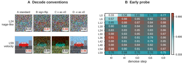
Figure 3: Decode convention flips; the probe reads early. A: four car_red decodes reverse convention between L24 and L59. B: a requested-color basis diagnostic reaches 0.883 patch-token accuracy at L6/t4 while the frozen head still reads noise (chance 0.33). Patches are not independent experimental units; the generation-level fixed-prompt result is 0.667 over 48 generations.
