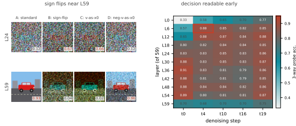
Figure 3: Left: four ways of turning an intermediate layer’s frozen-head output into an image for car_red at t=4 (A: standard \hat{x}_0=x_t-\sigma_tv_\ell ; B: sign-flipped; C: v_\ell decoded directly; D: -v_\ell decoded directly) – at L24 the standard decode is wrong-colored while the sign-flipped/direct decodes already look red, and at L59 this reverses. Right: cross-seed 3-way probe accuracy (chance = 0.33) by layer/step; the headline cell L6/t4 (0.883) is far above the frozen-head reading at the same cell, and probe accuracy drops at L59 relative to L48–L54.
