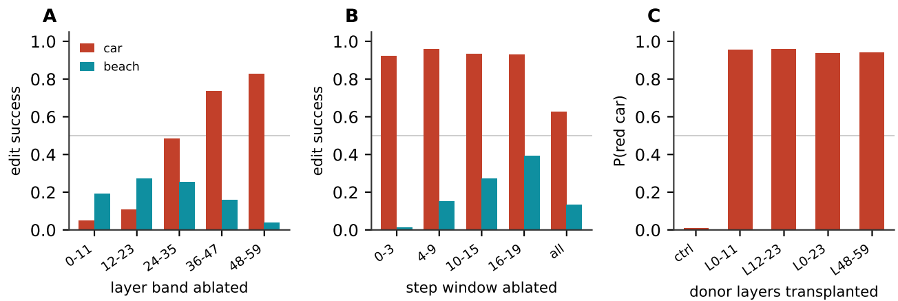
Figure 6: Causal ablation and transplant, car_red vs. beach_background . A : ablating a band of layers shows opposite profiles – car needs its early layers, beach needs its late ones. B : ablating a window of steps shows car tolerates any single window, beach is destroyed by ablating the earliest one. C : transplanting a donor car_red run’s hidden state into a car_green recipient, at any of four layer bands, is sufficient to flip the output back to red – including the L48–59 band, which panel A shows is not necessary for the car edit at all.
