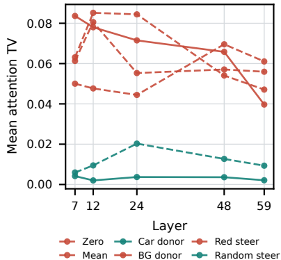
C Distortion by layer
