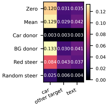
B Distortion by query group
