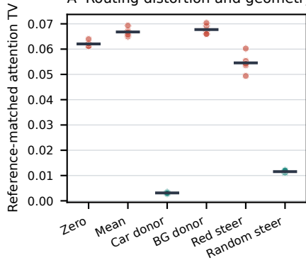
A Routing distortion and geometry
