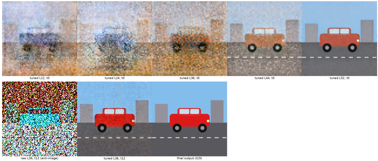
Figure 4: Internal image vs. frozen-head ghost. Top: tuned lens (fit on non-color edits, zero-shot on car_red ) decodes a coherent scene at every depth at t=0 . Bottom: at t=12 , the frozen head on the same L36 state is a color-inverted ghost; the tuned lens is coherent.
