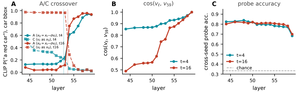
Figure 5: Translation band L52–54. Dense L44–L59 sweep on car_red . A : standard vs. direct- v CLIP scores cross in the band (both steps). B : \cos(v_L, v_{59}) rises sharply. C : probe accuracy stays flat through L58 and drops at L59 only.
