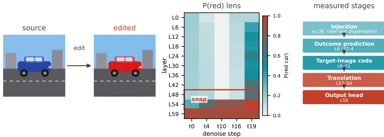
Figure 1: Predictable early, translated late. Center: frozen-head P(\text{red car}) on car_red across layer and step (snap L48–54). Right: five measured stages— injection , early outcome prediction , target-image code , L52–54 translation , L59 readout . Probes (not shown) predict the realized color from L6 while the head still reads noise.
