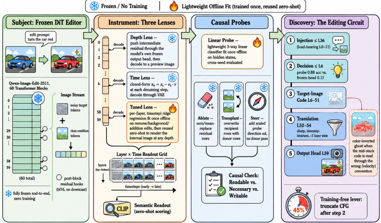
Figure 2: Layer–time instrument . Post-block residuals are hooked on the concatenated image stream. Depth lens : intermediate state \rightarrow frozen head \rightarrow decode. Time lens : step- t head output with \hat{x}_0 = x_t - \sigma_t v . Both use decode-then-CLIP readout on conditional and unconditional CFG passes alike.
