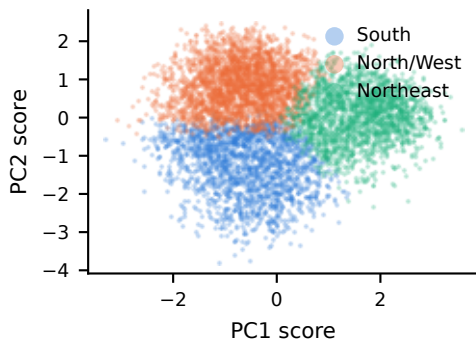
(c) k-means clusters on PC1 and PC2
