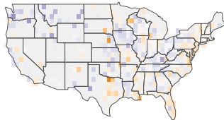
PC3 (2.8% of variance)
