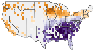
PC2 (3.3% of variance)
