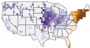
PC1 (4.2% of variance)
