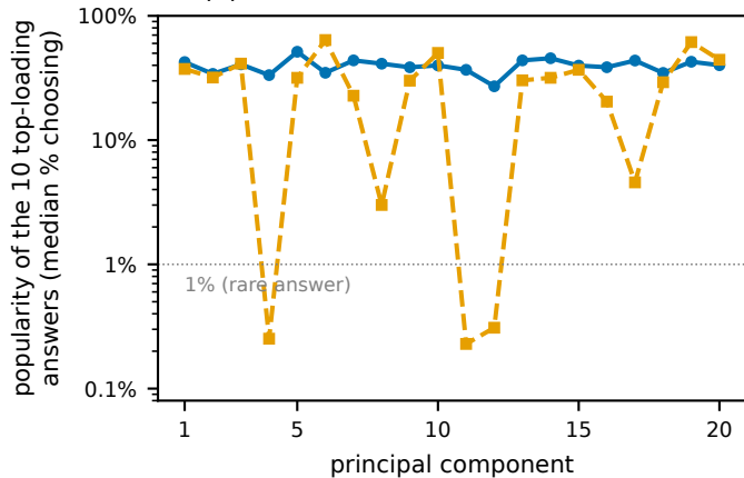
(b) what answers is each PC built on?
