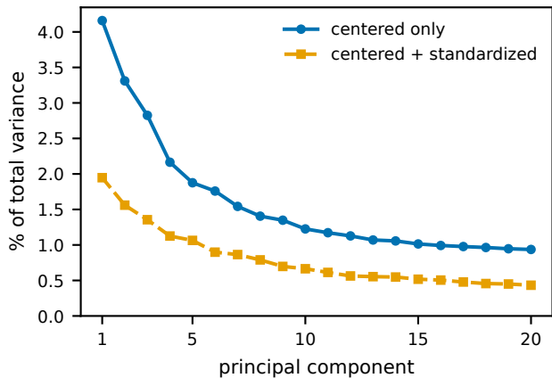
(a) scree plot
