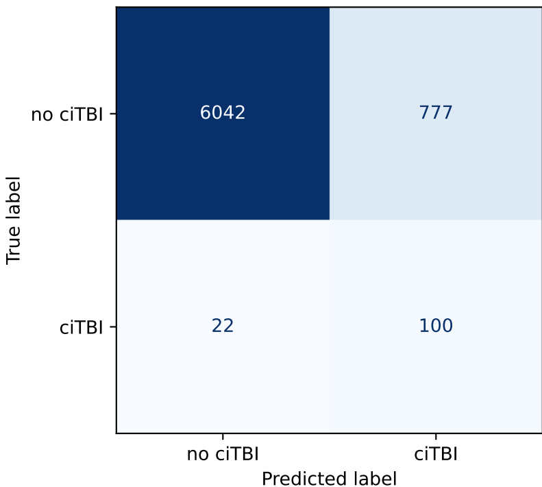
Baseline logistic regression (confusion matrix on train holdout)
