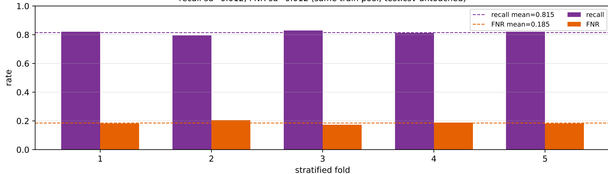
Data perturbation — stratified 5-fold CV of logistic L2 (preverbal/verbal) recall sd=0.012, FNR sd=0.012 (same train pool; test.csv untouched)
