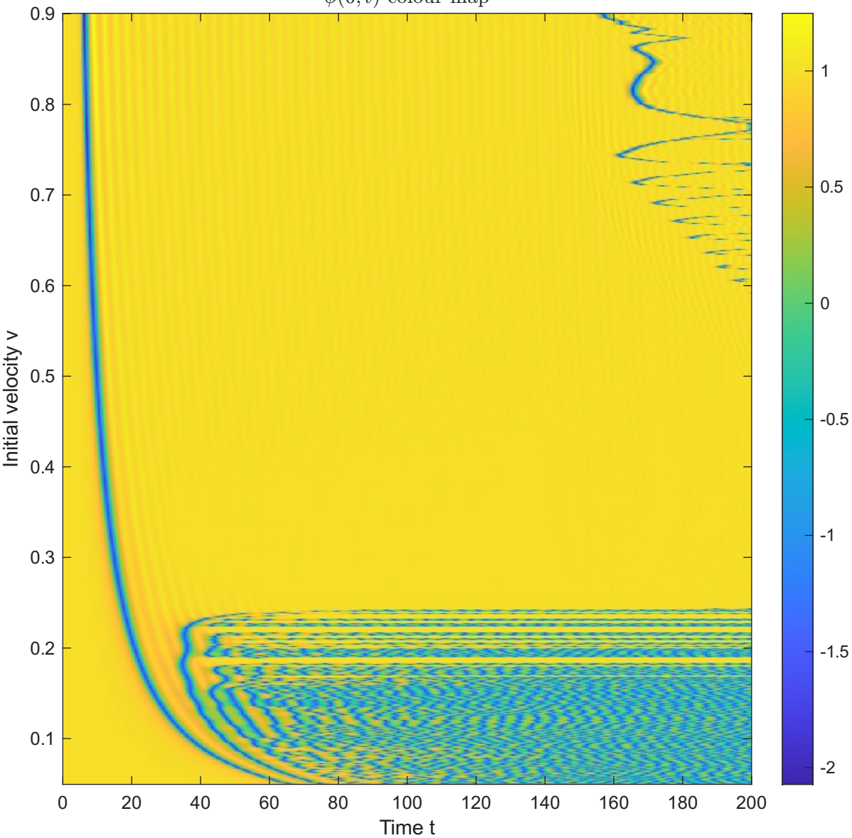
\phi(0, t) colour map
