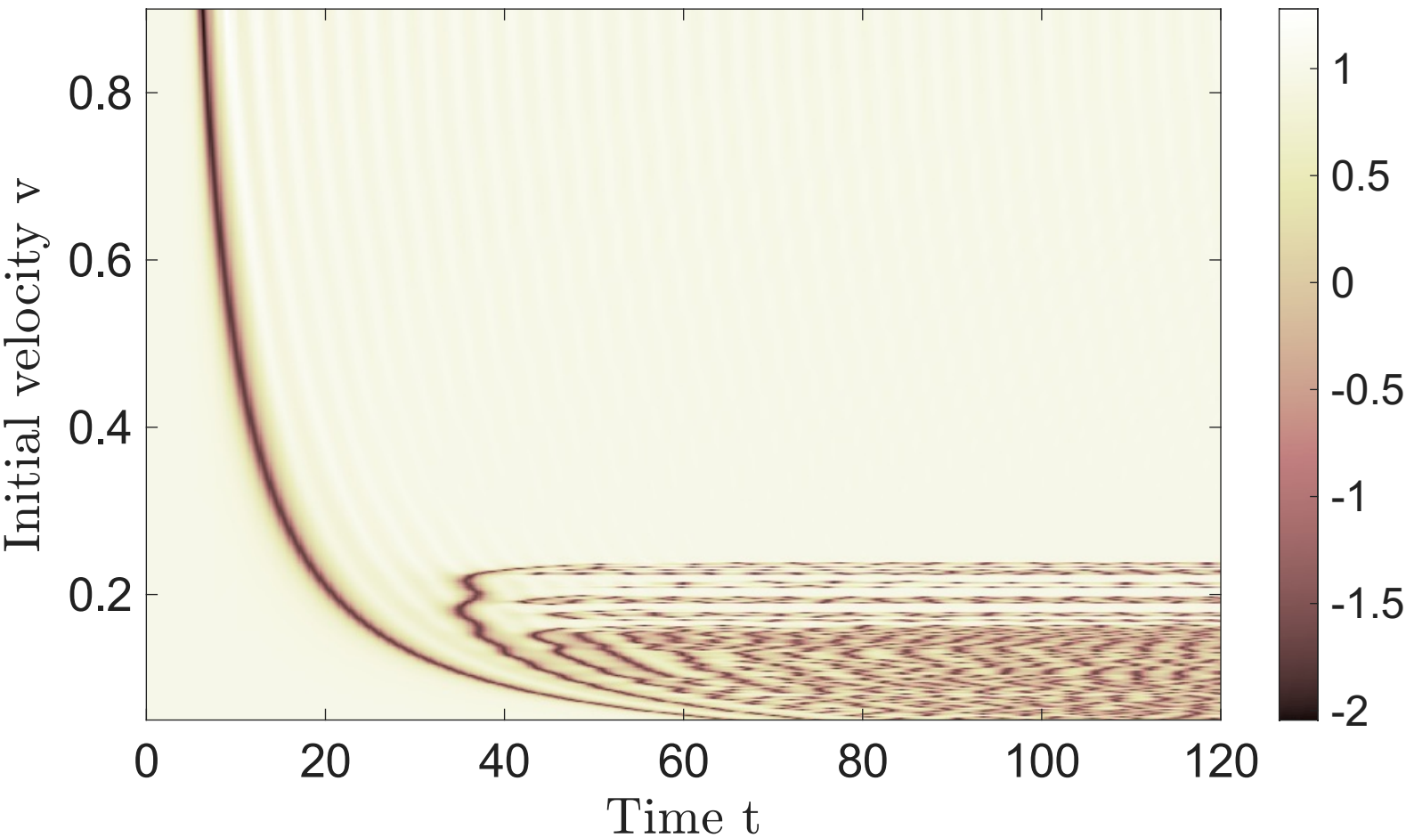
\phi(0, t) colour map
