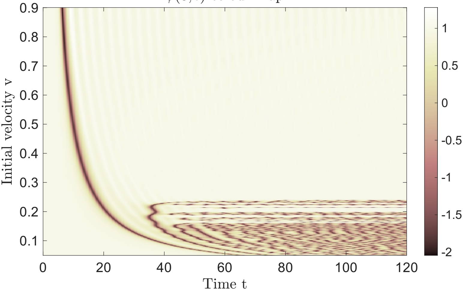
\phi(0, t) colour map
