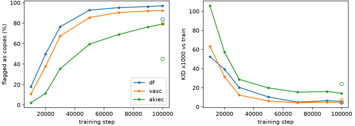
Figure 3. Left: lesion-calibrated flag rate. Right: KID x1000 vs train. Open markers: guidance 1.0 at 100k. Copying and train-referenced "quality" improve together, which is exactly why train-referenced quality cannot be trusted here.
