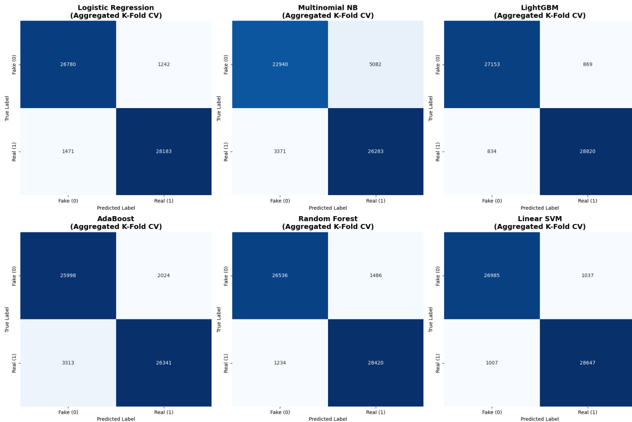
Confusion Matrices from Stratified K-Fold Cross-Validation
