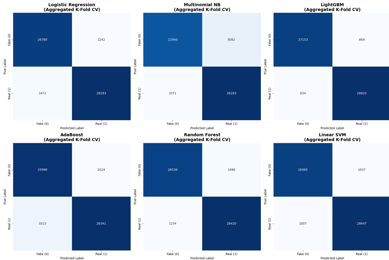
Confusion Matrices from Stratified K-Fold Cross-Validation
