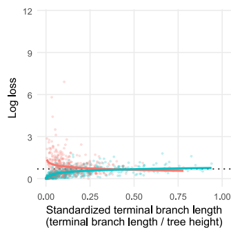
Q_{11}
