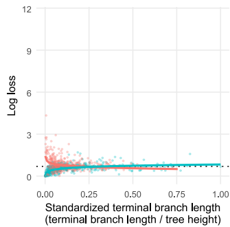
Q_6
