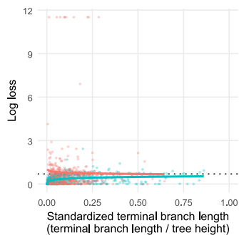
Q_{12}
