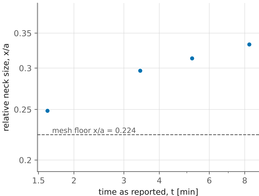
(a) Kingery (1960), T = -17.8\text{ }^{\circ}\text{C} , a = 110\text{ }\mu\text{m}
