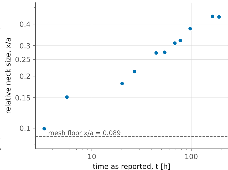
(b) Thomas et al. (1994), T = -20\text{ }^{\circ}\text{C} , a \approx 120\text{ }\mu\text{m}
