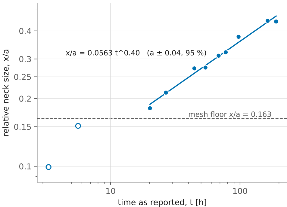
(a) Thomas et al. (1994), -20\text{ }^{\circ}\text{C} , a \approx 120\text{ }\mu\text{m}
