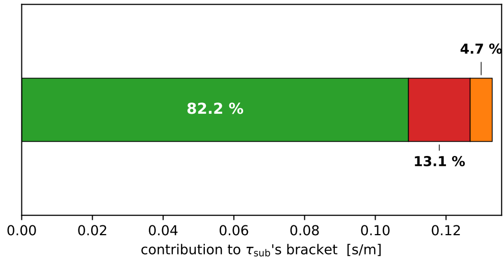
Anatomy of \tau_{\text{sub}} at \varepsilon = 8.58 \times 10^{-7} m, -20^\circ\text{C}
