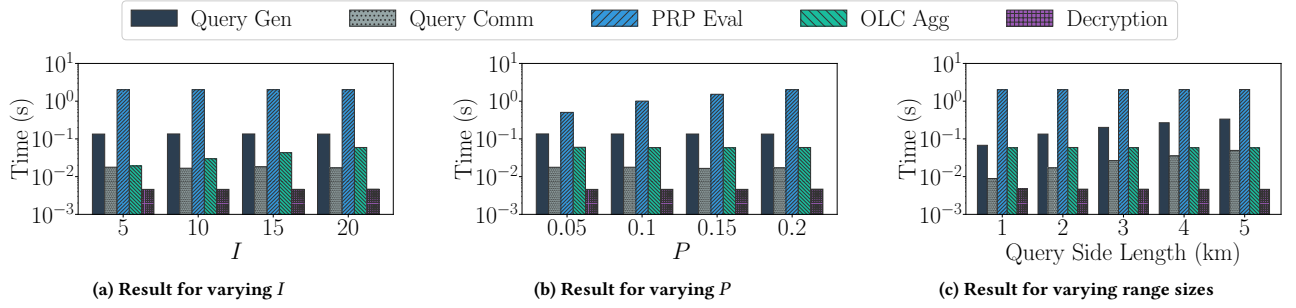
Figure 14: Detailed runtime analysis of PPRC under varying system parameters.
