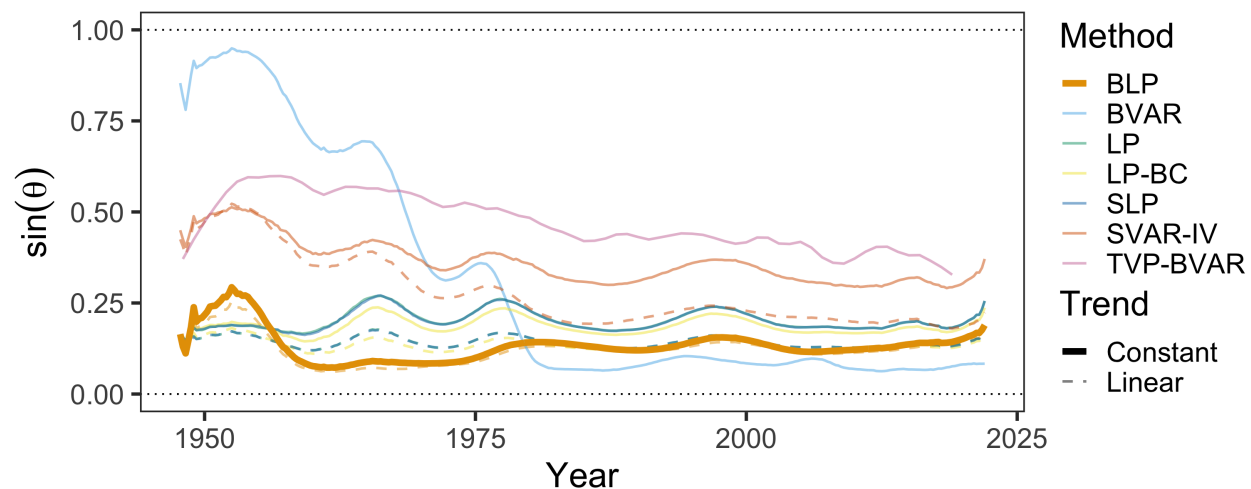
Figure F.4: Evolution of \sin \theta Across Methods
