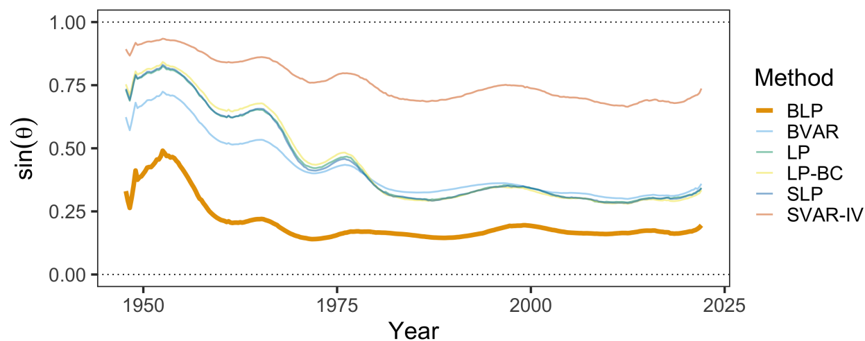
Figure G.5: Three-Instrument \sin \theta Across Estimation Methods
