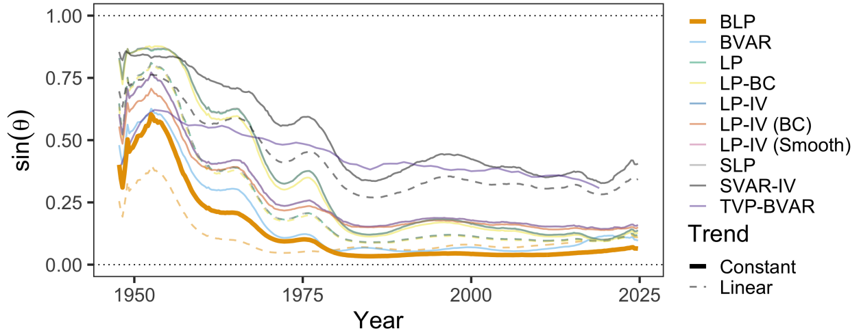
Figure D.1: Robustness Across Estimation Methodologies
