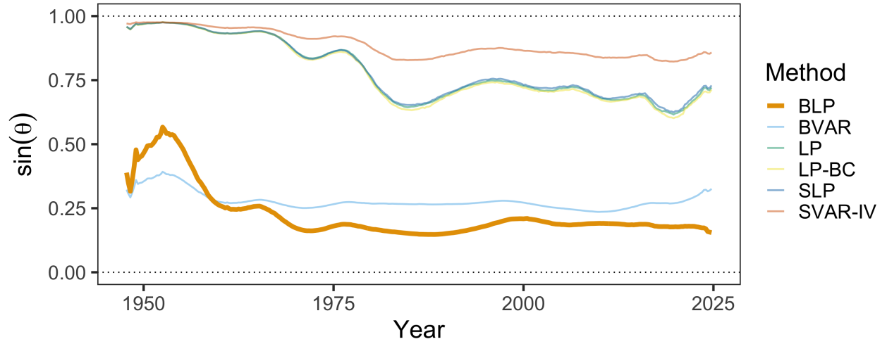
Figure G.1: Three-Instrument \sin \theta Across Estimation Methods
