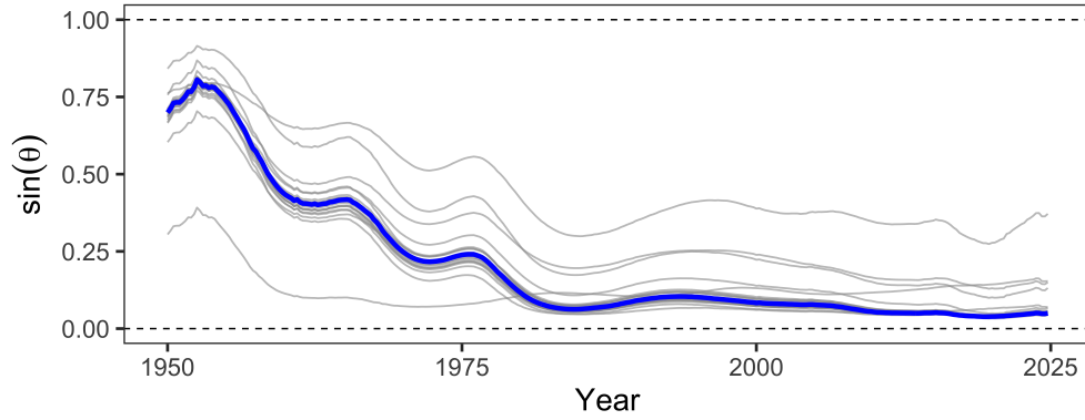
Figure D.6: Leave-One-Out Estimator for Bayesian LP
