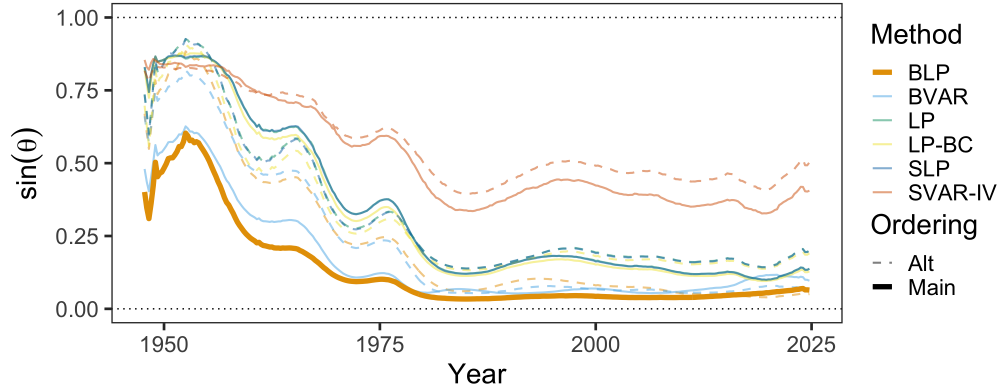
Figure D.4: Alignment with Reversed Cholesky Ordering
