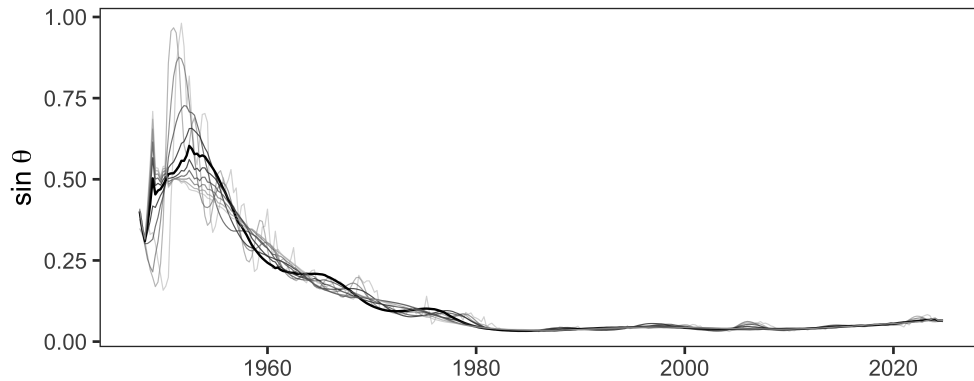
Figure D.5: Robustness to Filtering Choice
