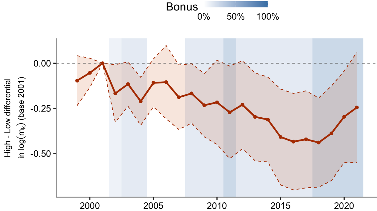
Figure 5: Calendar Difference-in-Differences
