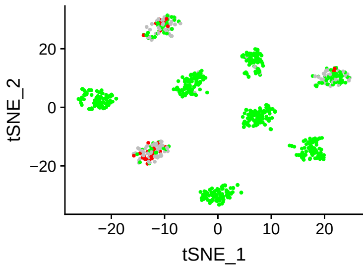
ENSG00000014641
