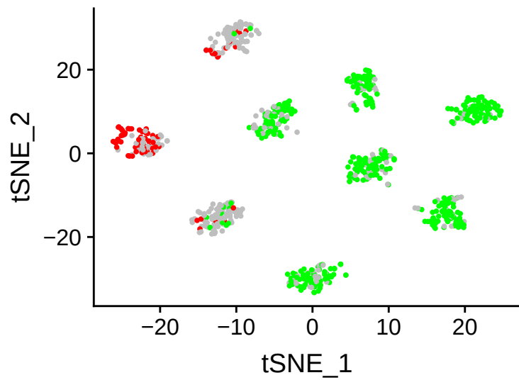
ENSG00000053438
