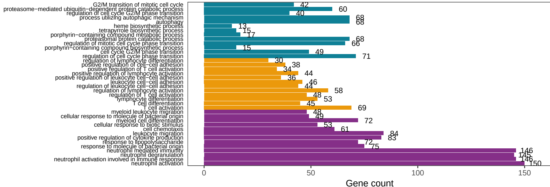
GO enrichment of cluster
